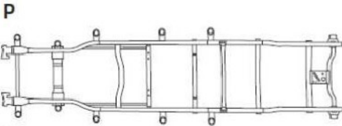
UNDERBODY VIEW
